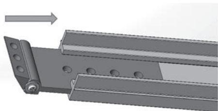
Drawings 18A & 18B: INSERT RAKE-LOC™ STAIR RAIL BRACKET ASSEMBLIES FOR TOP OF STAIRS & BOTTOM OF STAIRS INTO THE TOP ALUMINUM STIFFENER
