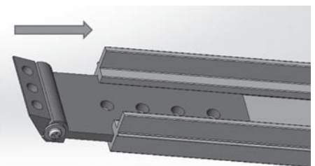
Drawings 8A & 8B: INSERT RAKE-LOC™ RAIL BRACKET ASSEMBLIES FOR TOP OF STAIRS & BOTTOM OF STAIRS INTO THE ALUMINUM STIFFENER
